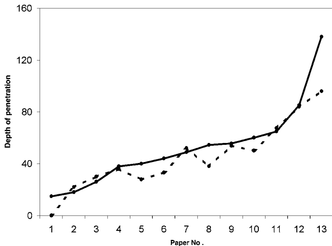
FIG. 3—Depth of penetration (microns) of DFO and 1,2-indanedione-treated prints, for 13 uncoated papers (—) DFO, (---) 1,2-indanedione.
