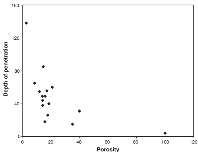
FIG. 5—Depth of fingerprint penetration (DFO, microns) vs. paper porosity (sec/100 cm 3 ) for 13 uncoated papers.
